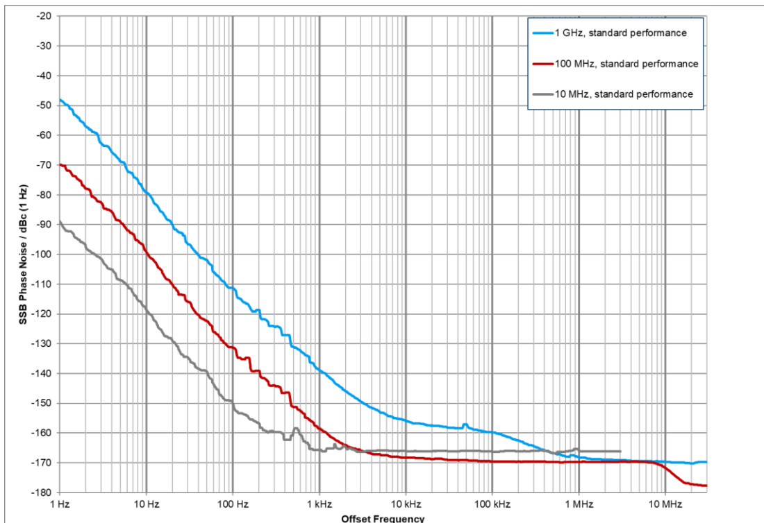
Measured SSB phase noise of reference outputs at f = 10 MHz, 100 MHz and 1 GHz ( f = 100 MHz and 1 GHz only available with the R&S ® SMAB-K703 option)
