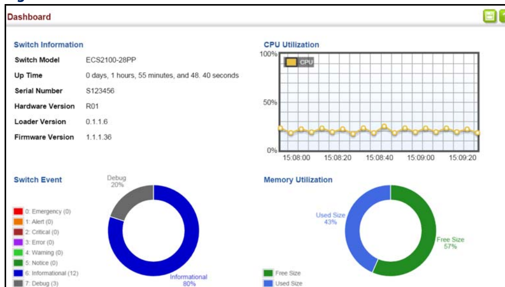
Figure 1: Dashboard
