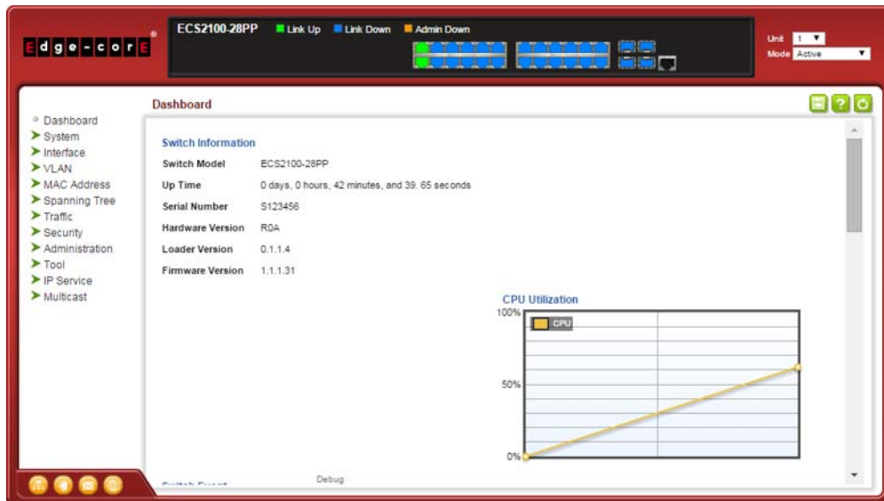
Figure 2: Home Page
