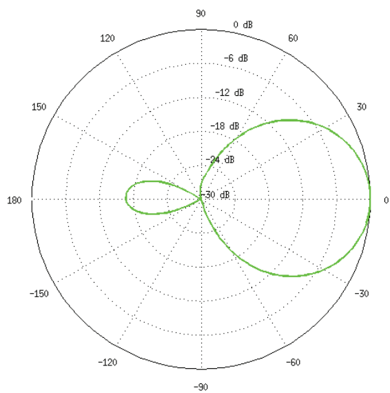
Horizontal Azimuth
