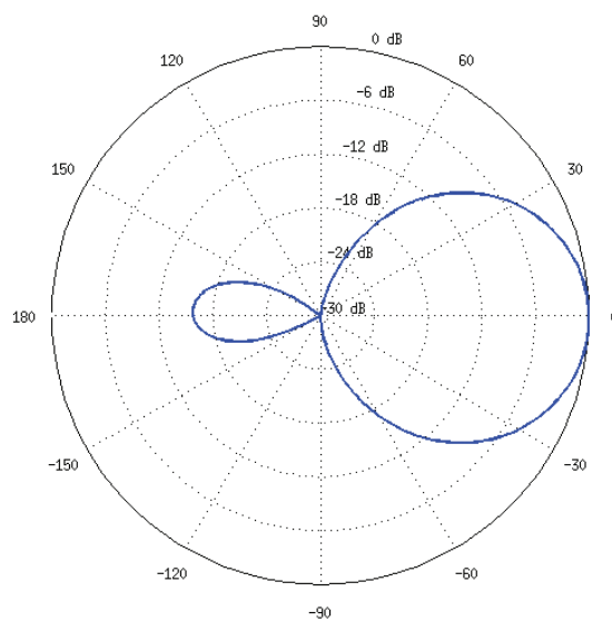
Horizontal Elevation
